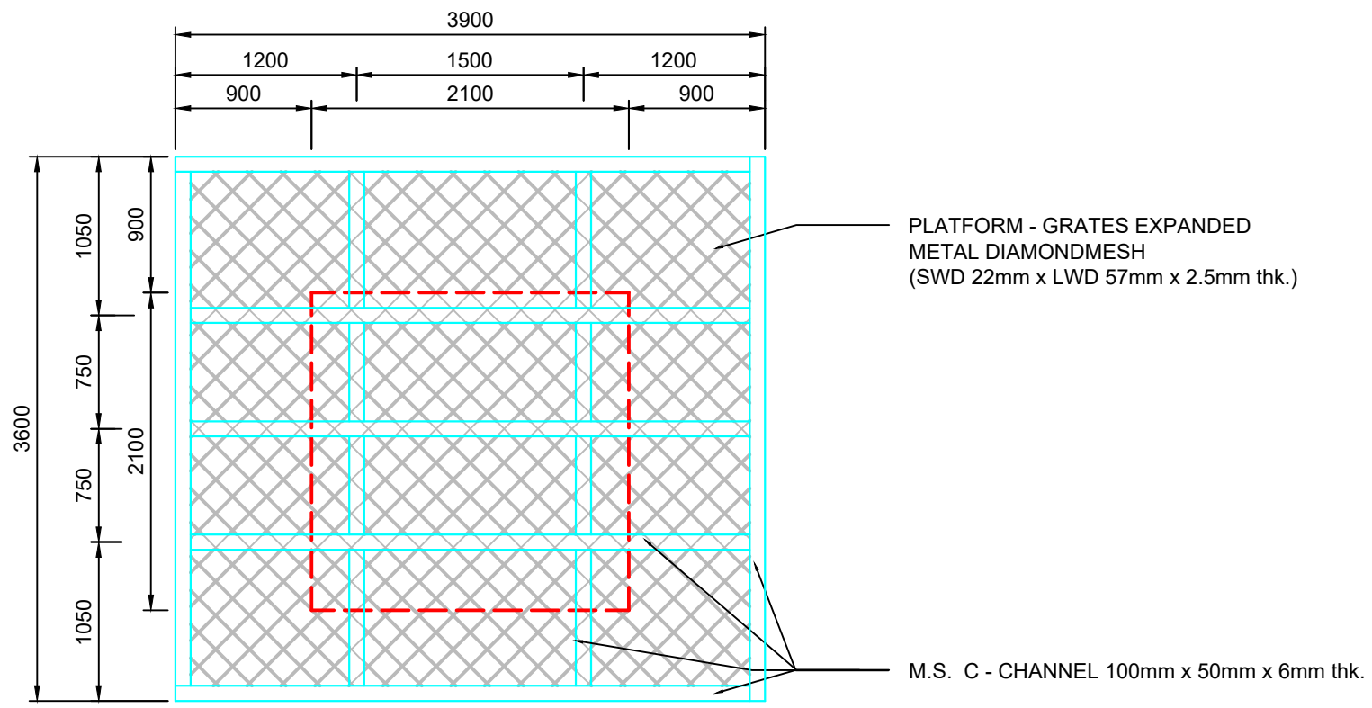
PLAN OF PLATFORM FOR 1 UNIT
